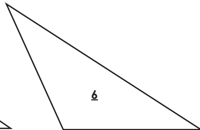
Obtuse Isosceles Triangle
