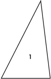
Acute Scalene Triangle
