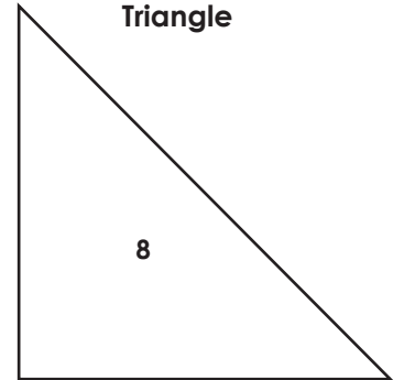
Large Right Isosceles Triangle
