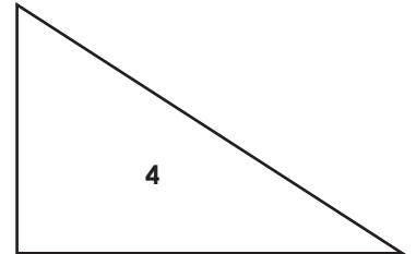
Right Scalene Triangle
