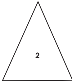
Acute Isosceles Triangle
