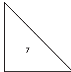
Small Right Isosceles Triangle
