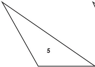
Obtuse Scalene Triangle
